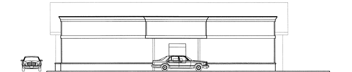
NORTH ELEVATION - (COVERED DRIVE THRU)
