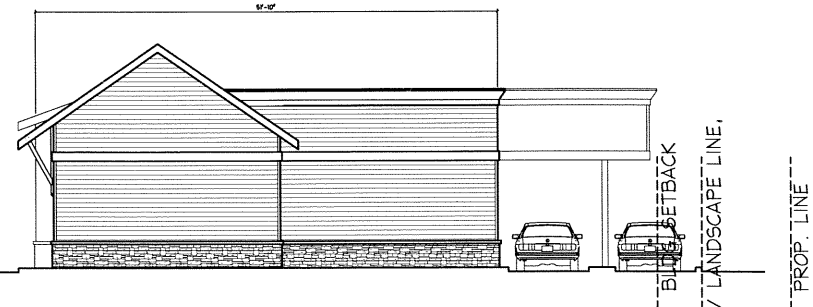
EAST ELEVATION - (COVERED 2-LANE DRIVE THRU)
